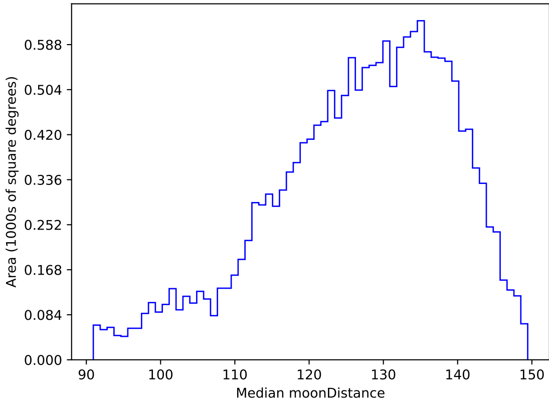
weather_cloudso0v3.5_10yrs WFD u band: Median moonDistance
