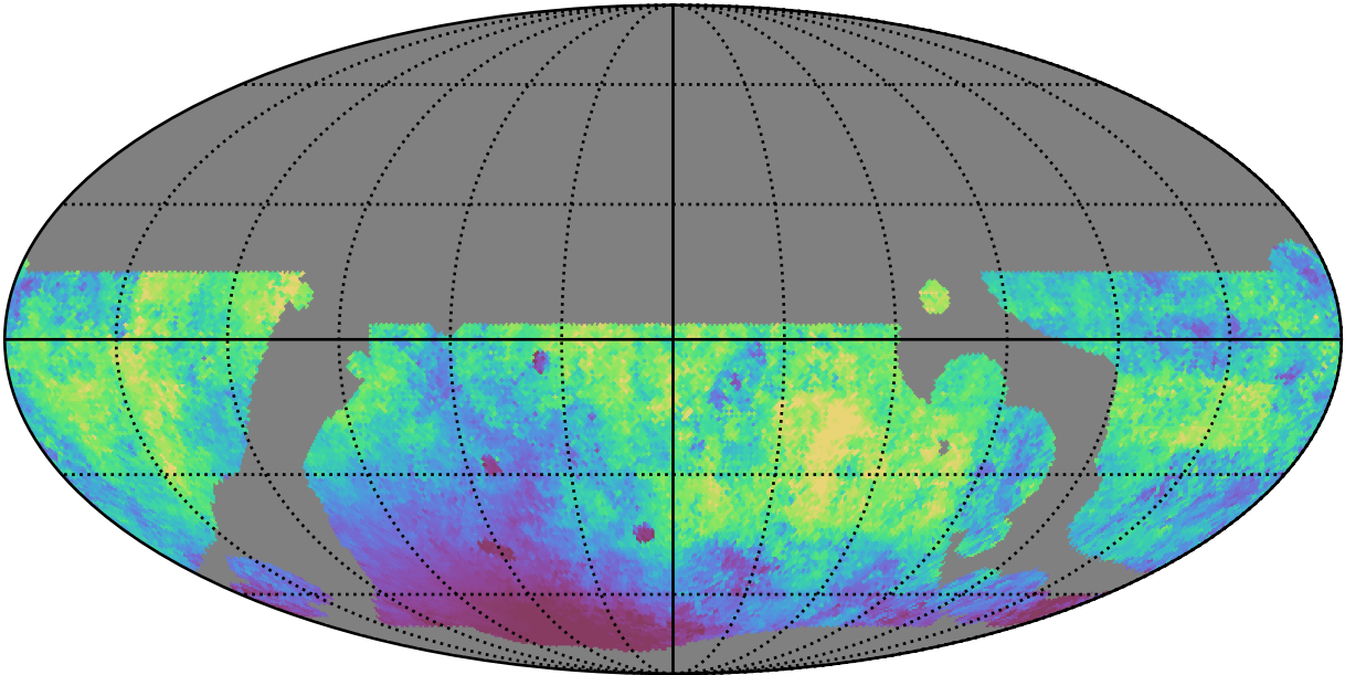
weather_cloudso0v3.5_10yrs WFD r band: Median moonDistance
