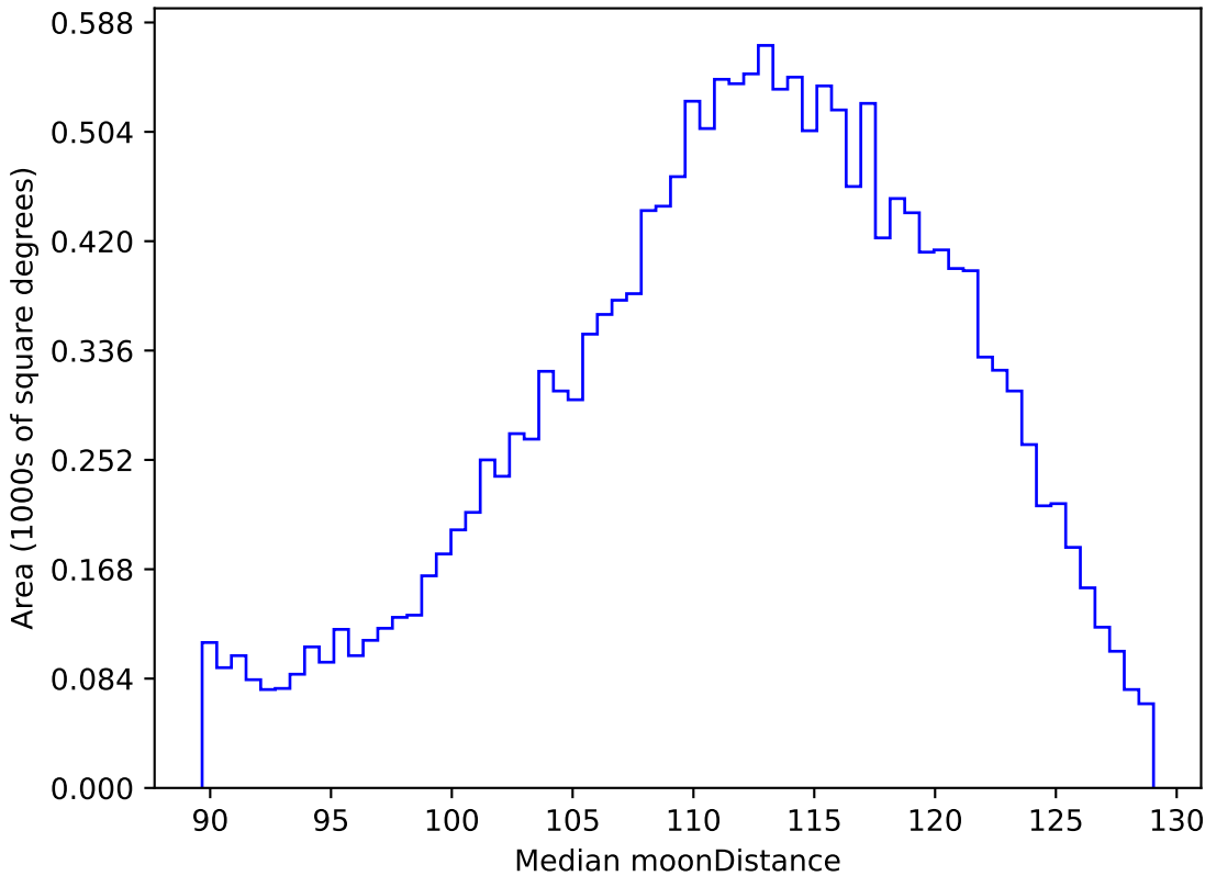
weather_cloudso0v3.5_10yrs WFD r band: Median moonDistance
