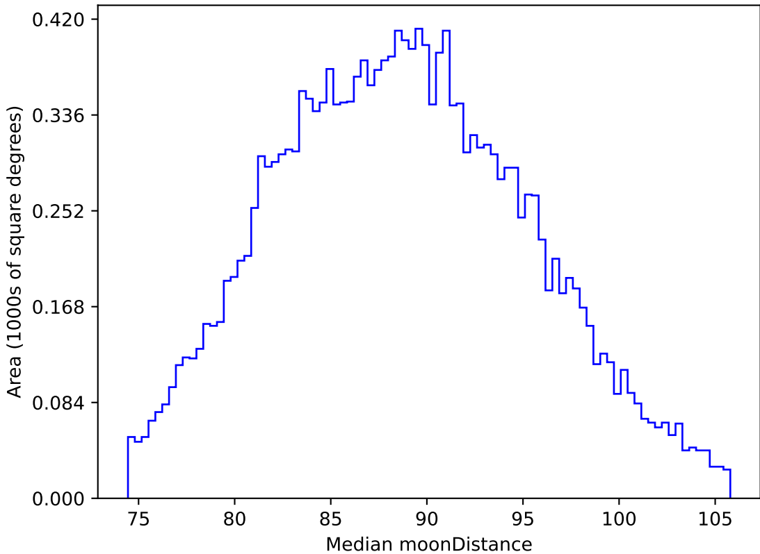
weather_cloudso0v3.5_10yrs WFD i band: Median moonDistance
