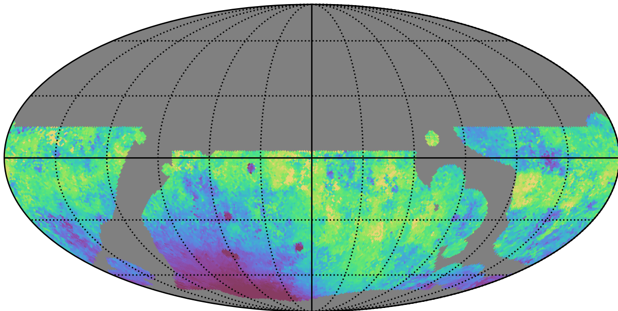
weather_cloudso0v3.5_10yrs WFD g band: Median moonDistance
