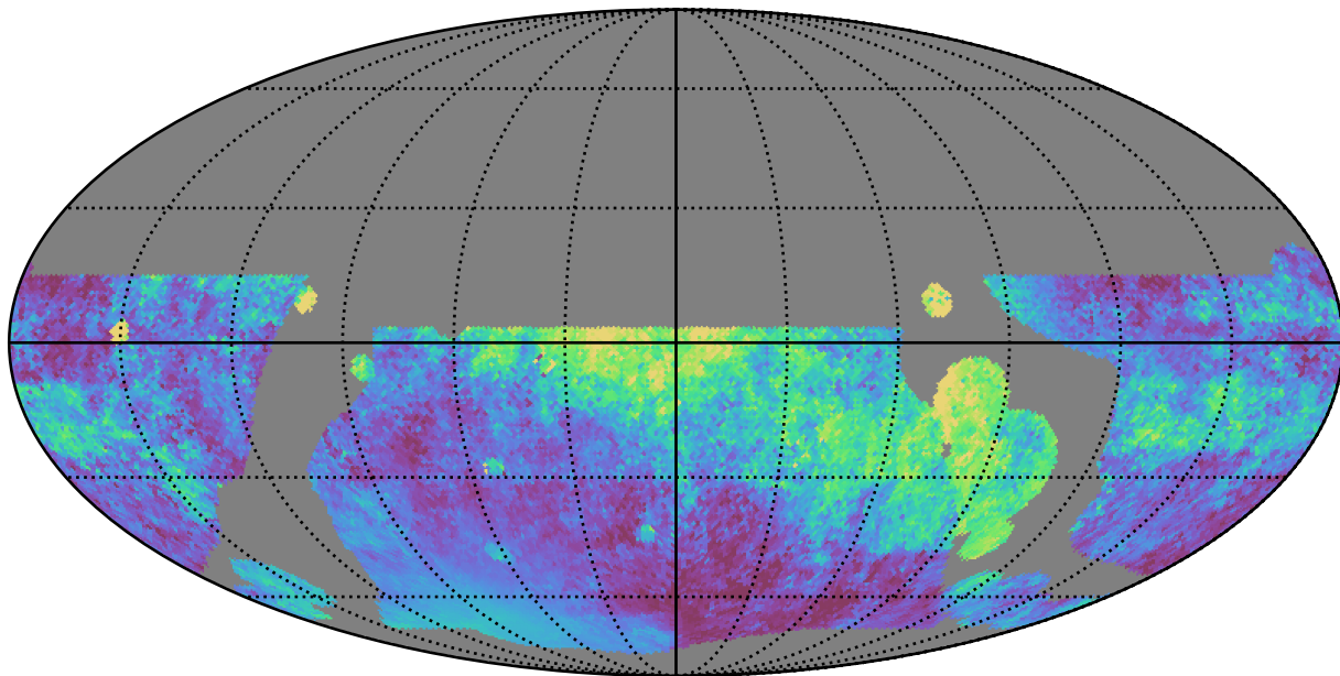
weather_cloudso0v3.5_10yrs WFD all bands: Median moonDistance
