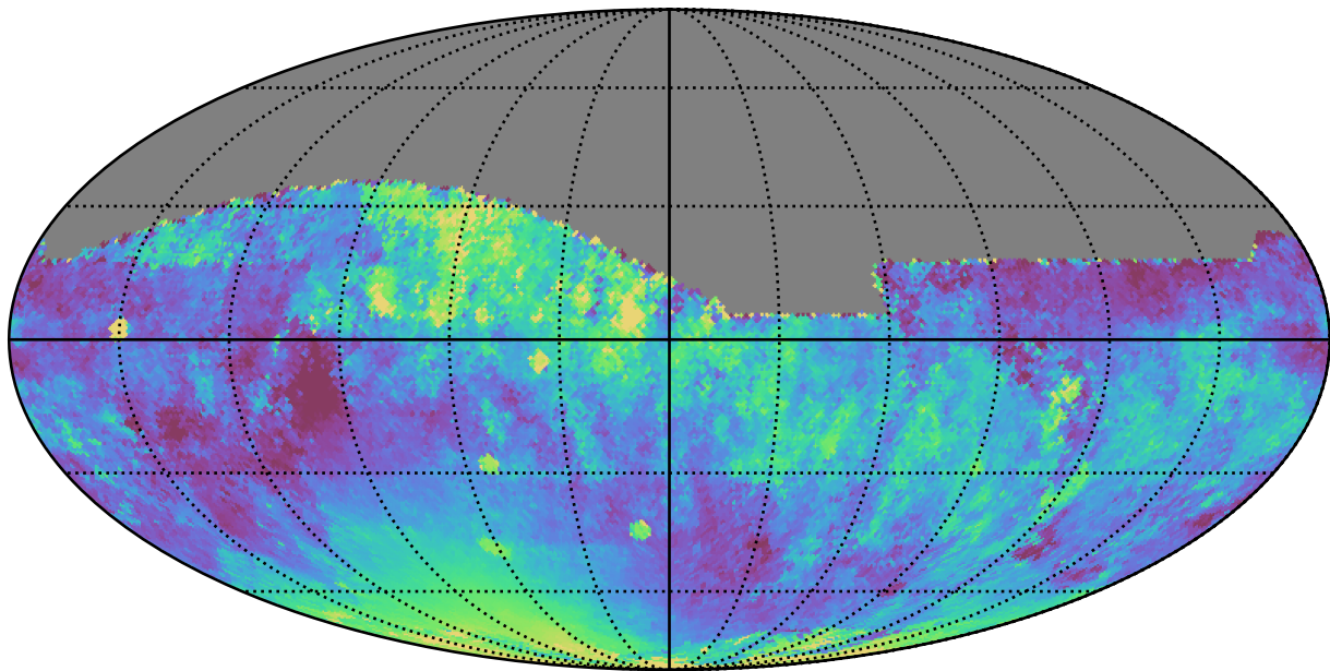
weather_cloudso0v3.5_10yrs All sky z band: Median moonDistance
