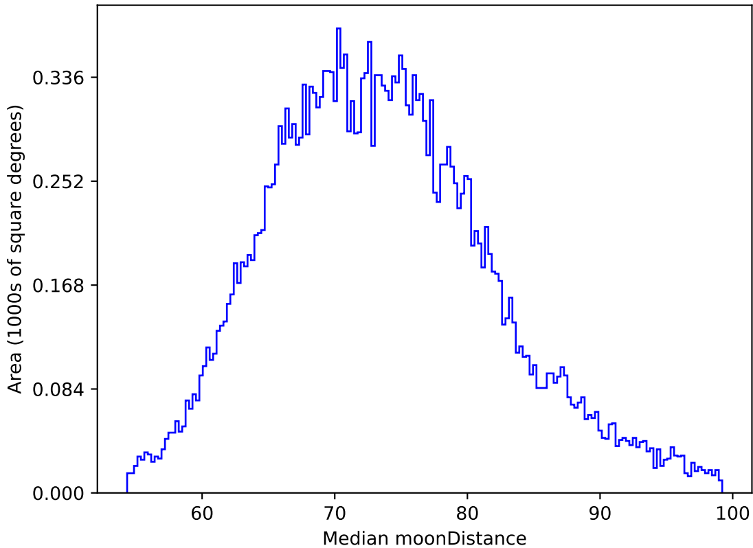
weather_cloudso0v3.5_10yrs All sky z band: Median moonDistance
