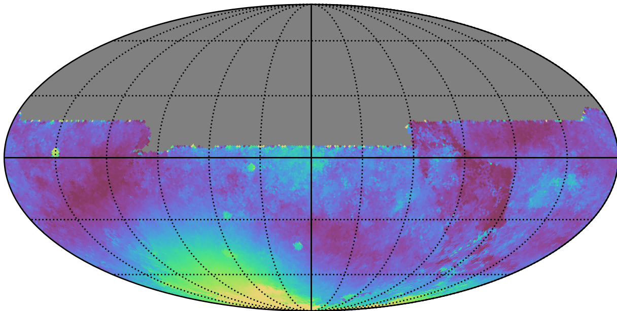
weather_cloudso0v3.5_10yrs All sky y band: Median moonDistance
