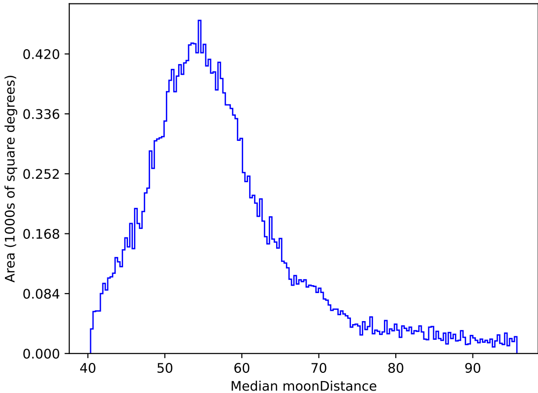
weather_cloudso0v3.5_10yrs All sky y band: Median moonDistance
