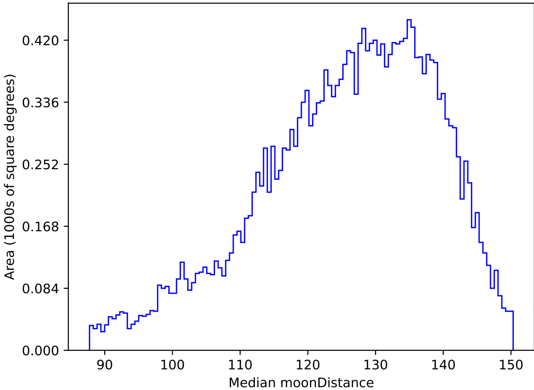
weather_cloudso0v3.5_10yrs All sky u band: Median moonDistance
