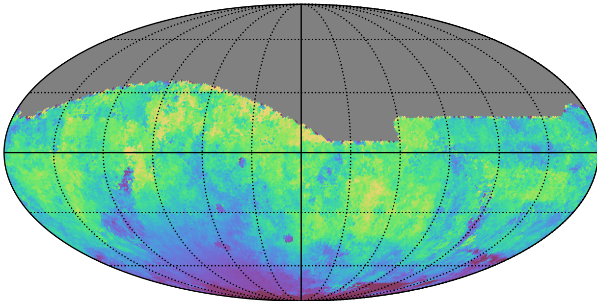
weather_cloudso0v3.5_10yrs All sky r band: Median moonDistance
