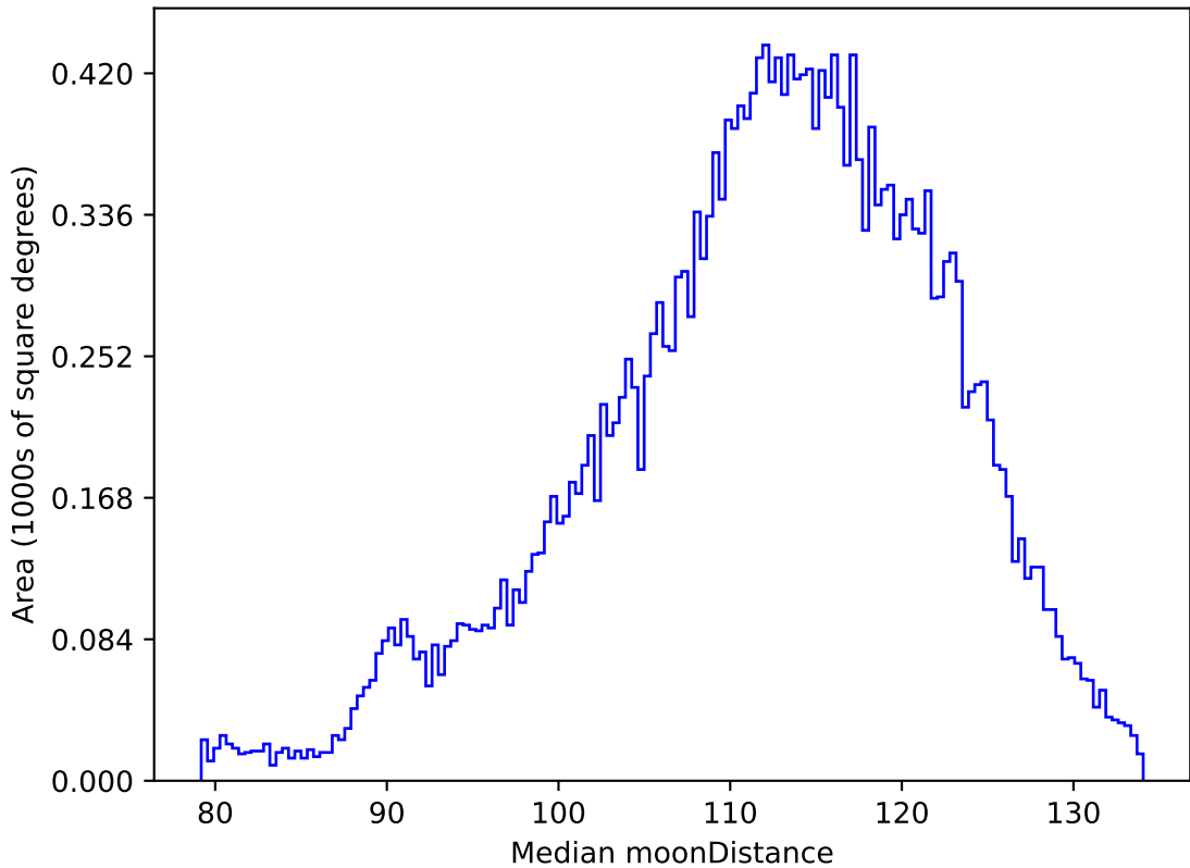
weather_cloudso0v3.5_10yrs All sky r band: Median moonDistance
