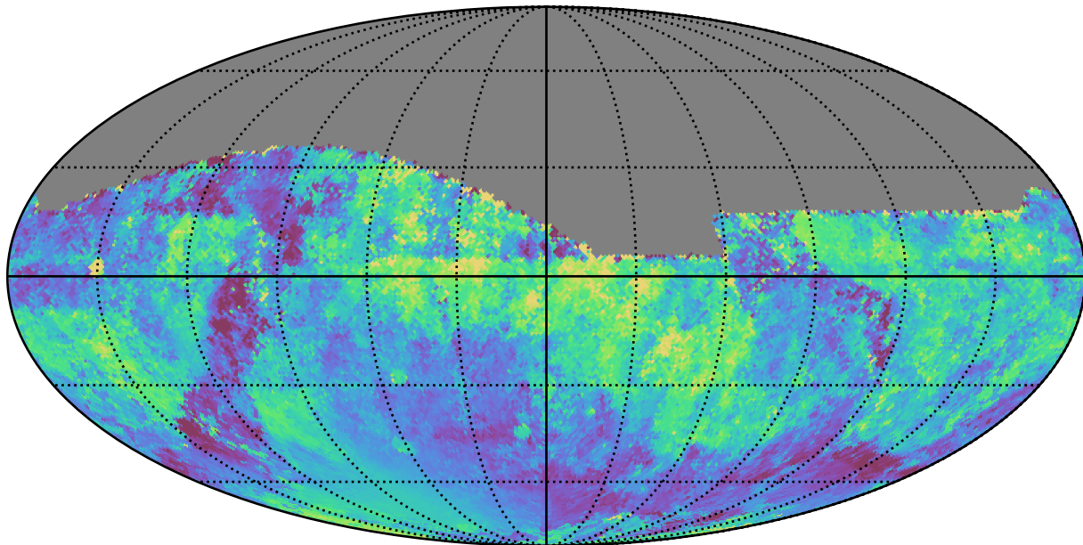
weather_cloudso0v3.5_10yrs All sky i band: Median moonDistance
