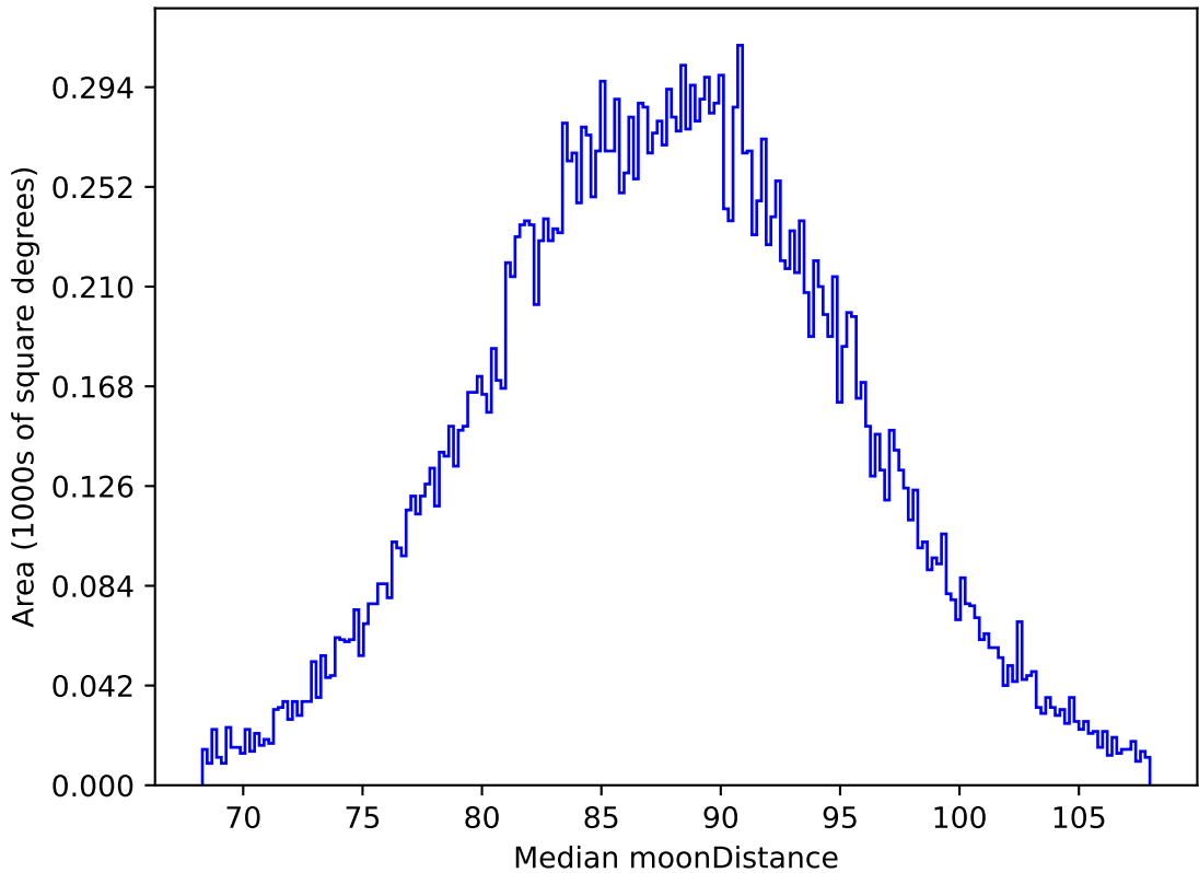
weather_cloudso0v3.5_10yrs All sky i band: Median moonDistance
