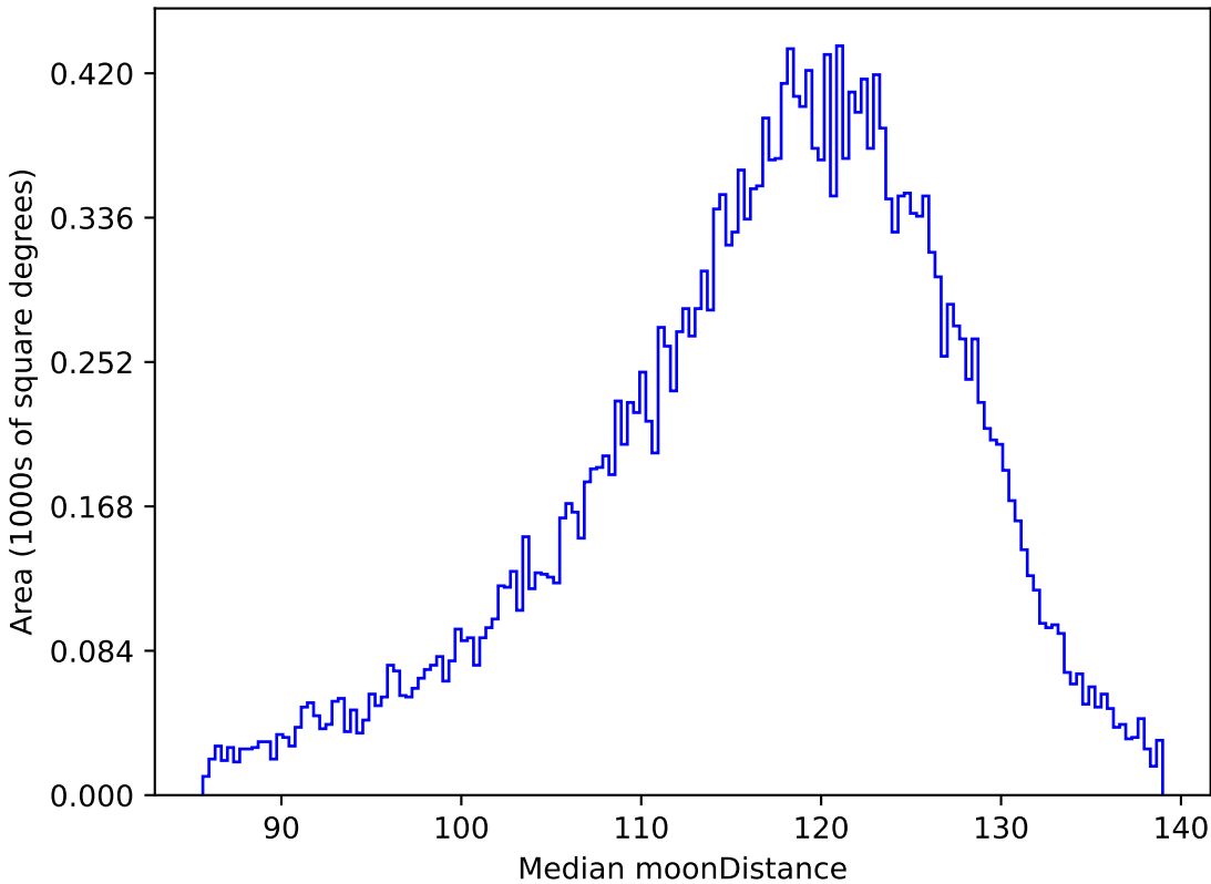
weather_cloudso0v3.5_10yrs All sky g band: Median moonDistance
