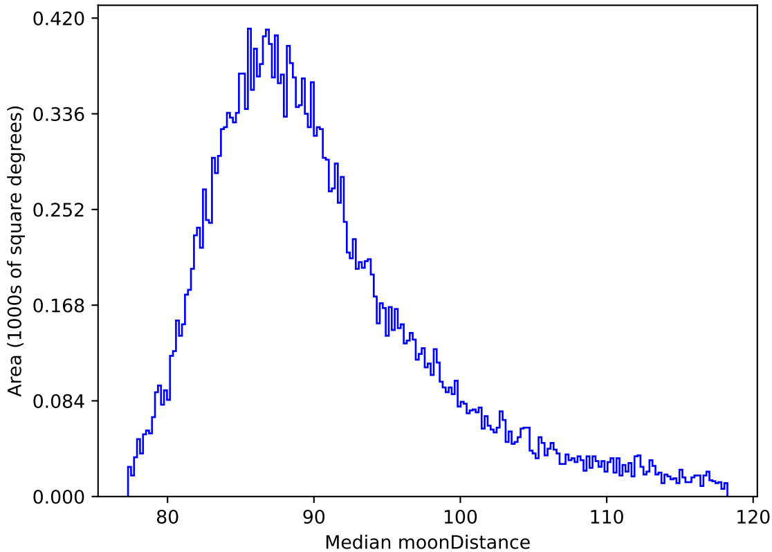
weather_cloudso0v3.5_10yrs All sky all bands: Median moonDistance
