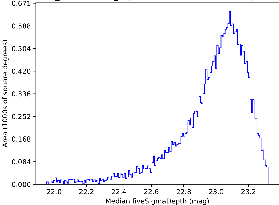
weather_cloudso0v3.5_10yrs Yr 1 z band: Median fiveSigmaDepth
