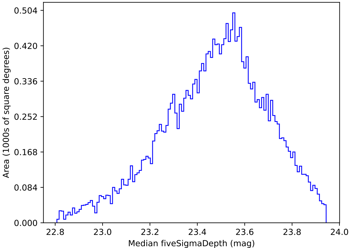
weather_cloudso0v3.5_10yrs Yr 1 u band: Median fiveSigmaDepth
