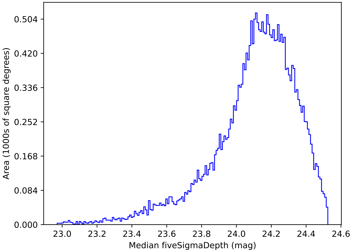
weather_cloudso0v3.5_10yrs Yr 1 r band: Median fiveSigmaDepth
