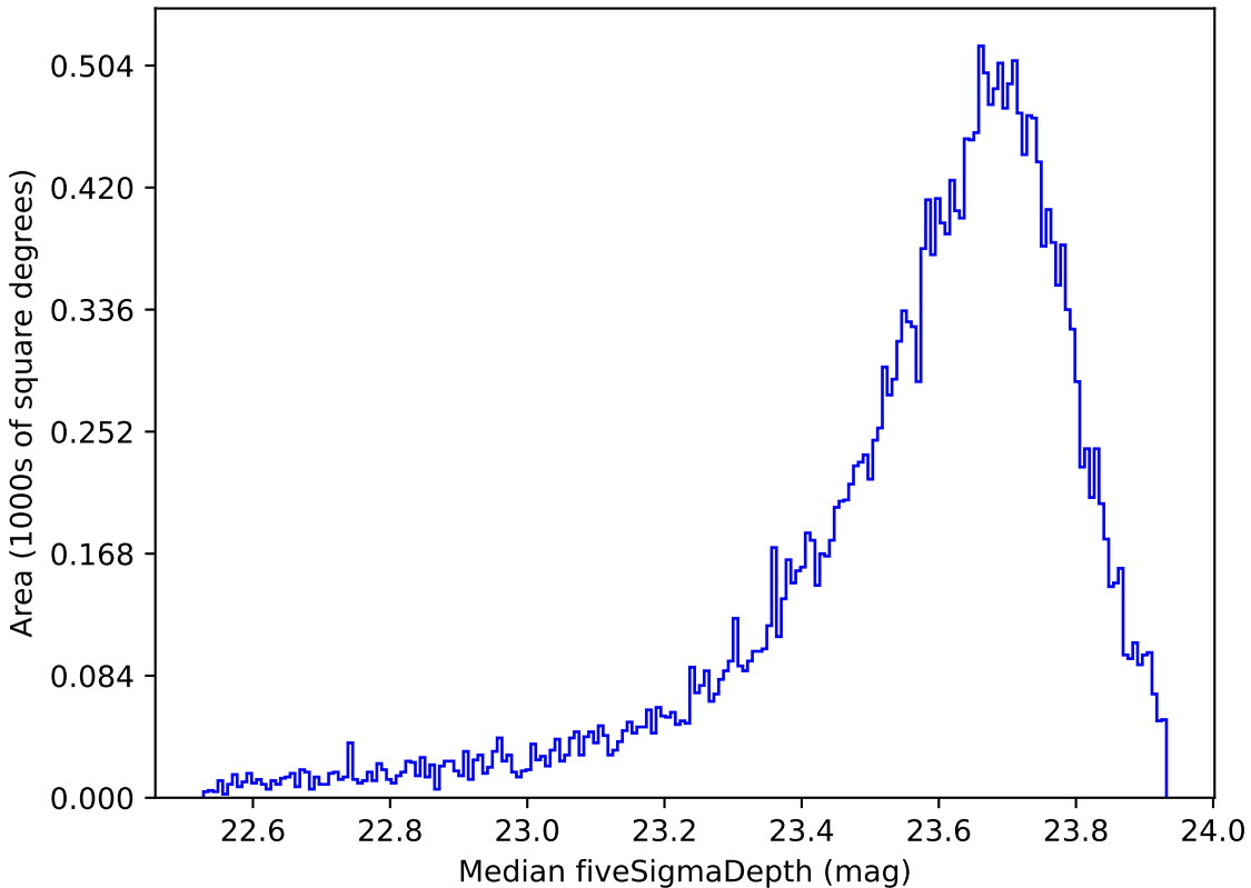
weather_cloudso0v3.5_10yrs Yr 1 i band: Median fiveSigmaDepth
