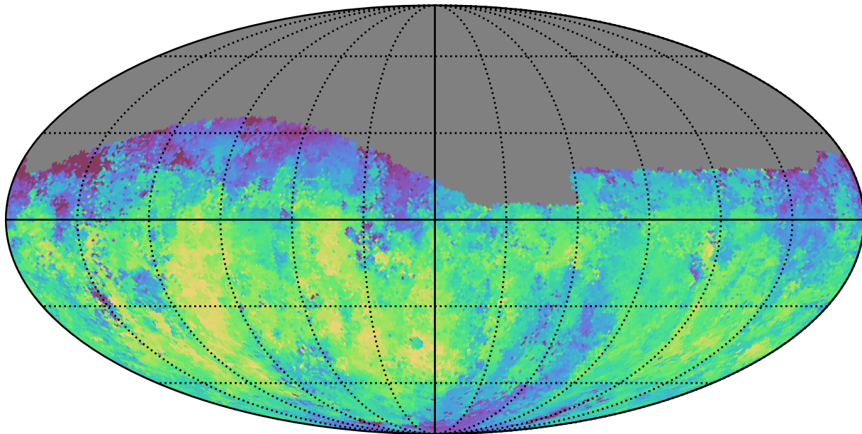
weather_cloudso0v3.5_10yrs Yr 1 g band: Median fiveSigmaDepth
