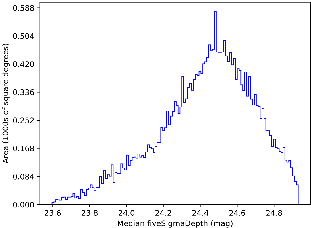
weather_cloudso0v3.5_10yrs Yr 1 g band: Median fiveSigmaDepth
