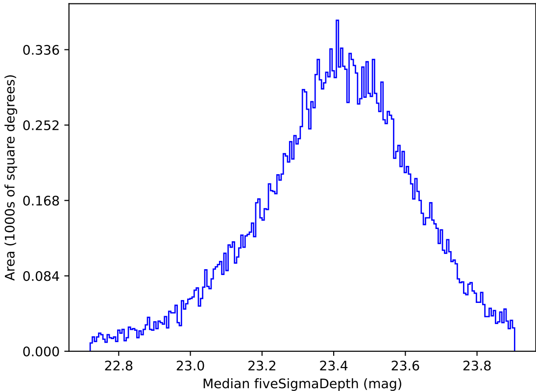
weather_cloudso0v3.5_10yrs Yr 1 all bands: Median fiveSigmaDepth
