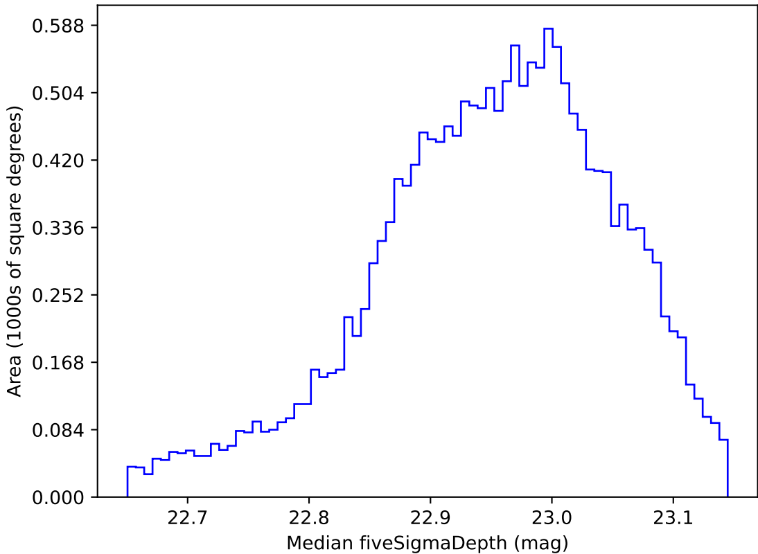
weather_cloudso0v3.5_10yrs WFD z band: Median fiveSigmaDepth
