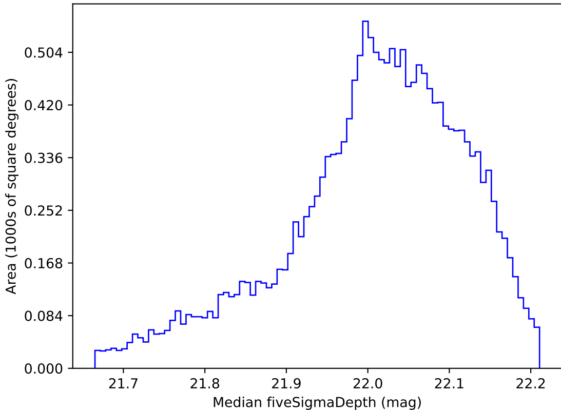
weather_cloudso0v3.5_10yrs WFD y band: Median fiveSigmaDepth
