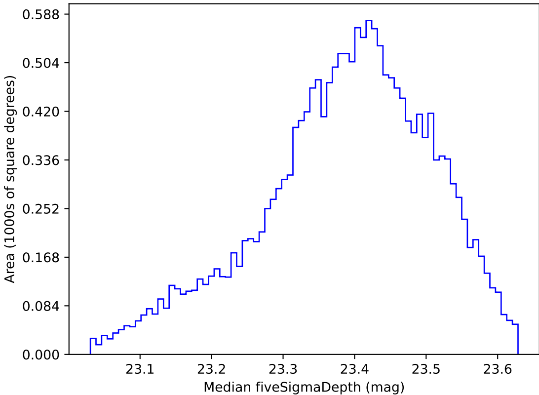
weather_cloudso0v3.5_10yrs WFD u band: Median fiveSigmaDepth
