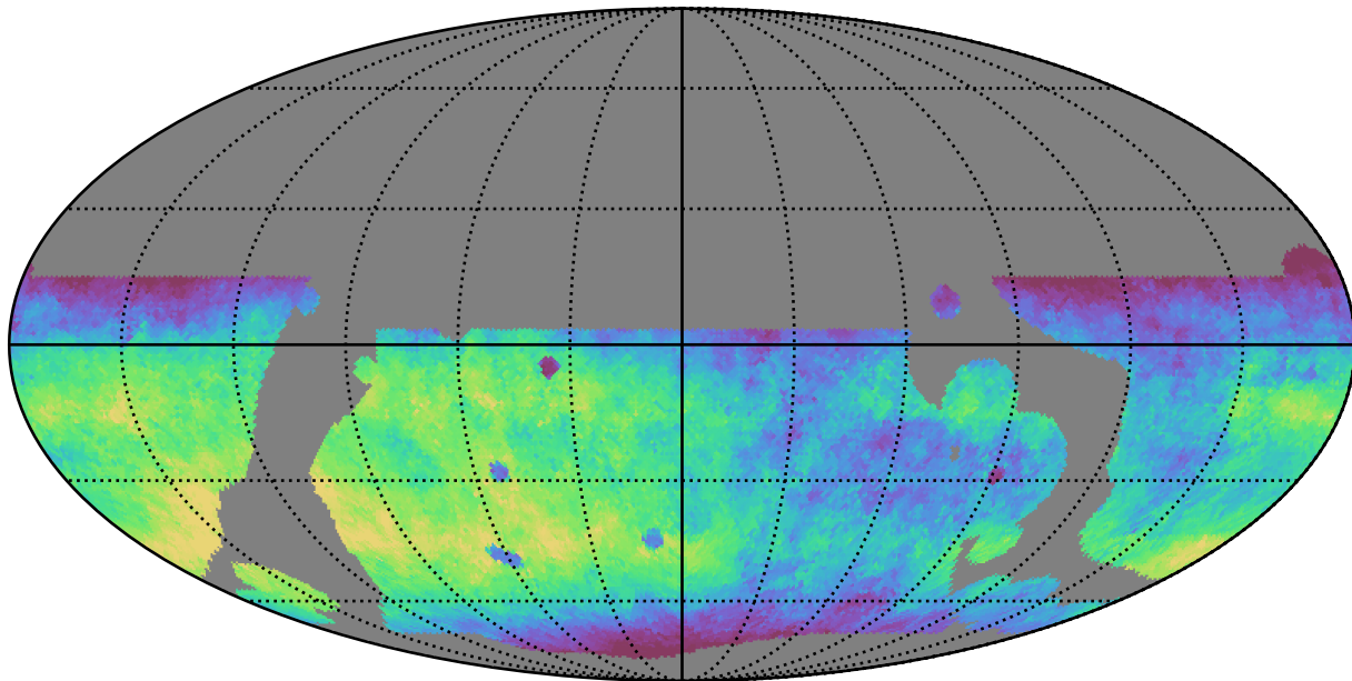
weather_cloudso0v3.5_10yrs WFD r band: Median fiveSigmaDepth
