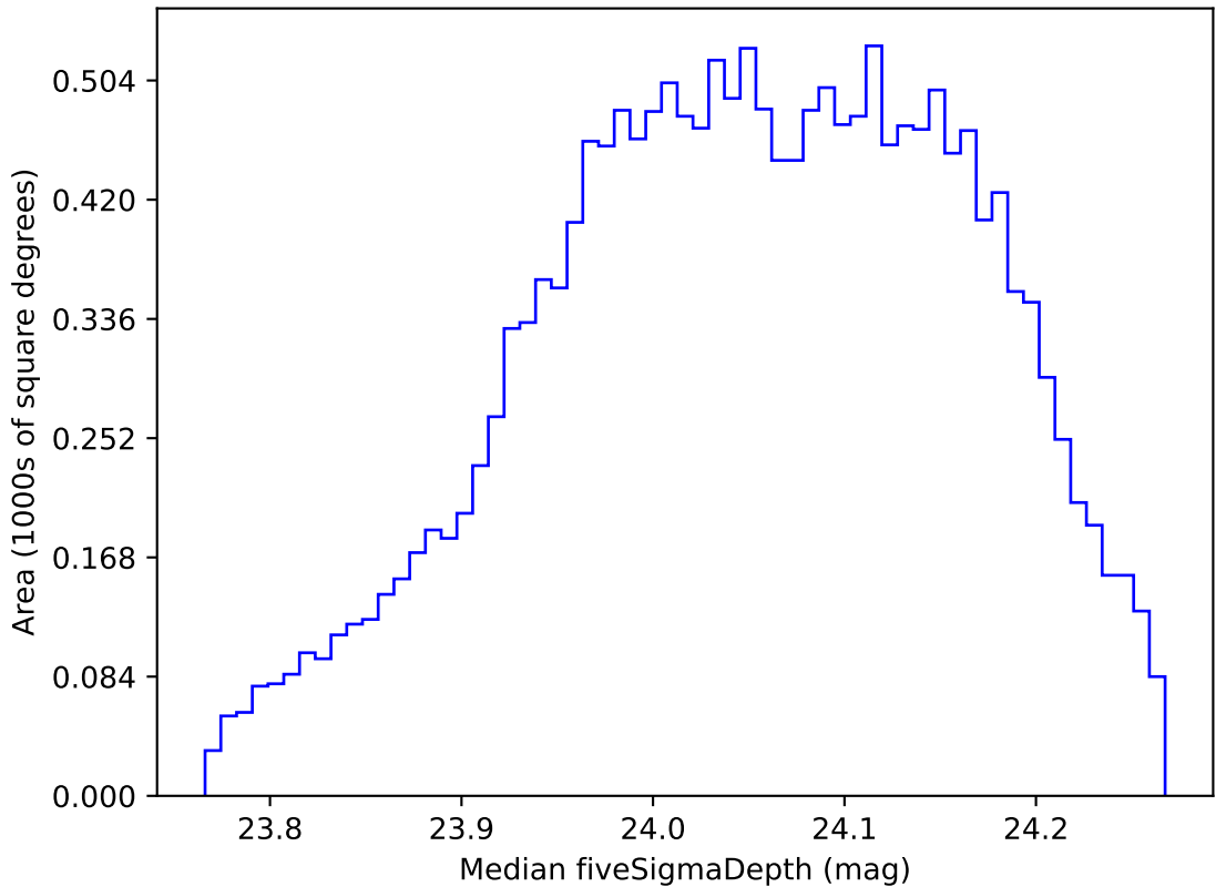
weather_cloudso0v3.5_10yrs WFD r band: Median fiveSigmaDepth
