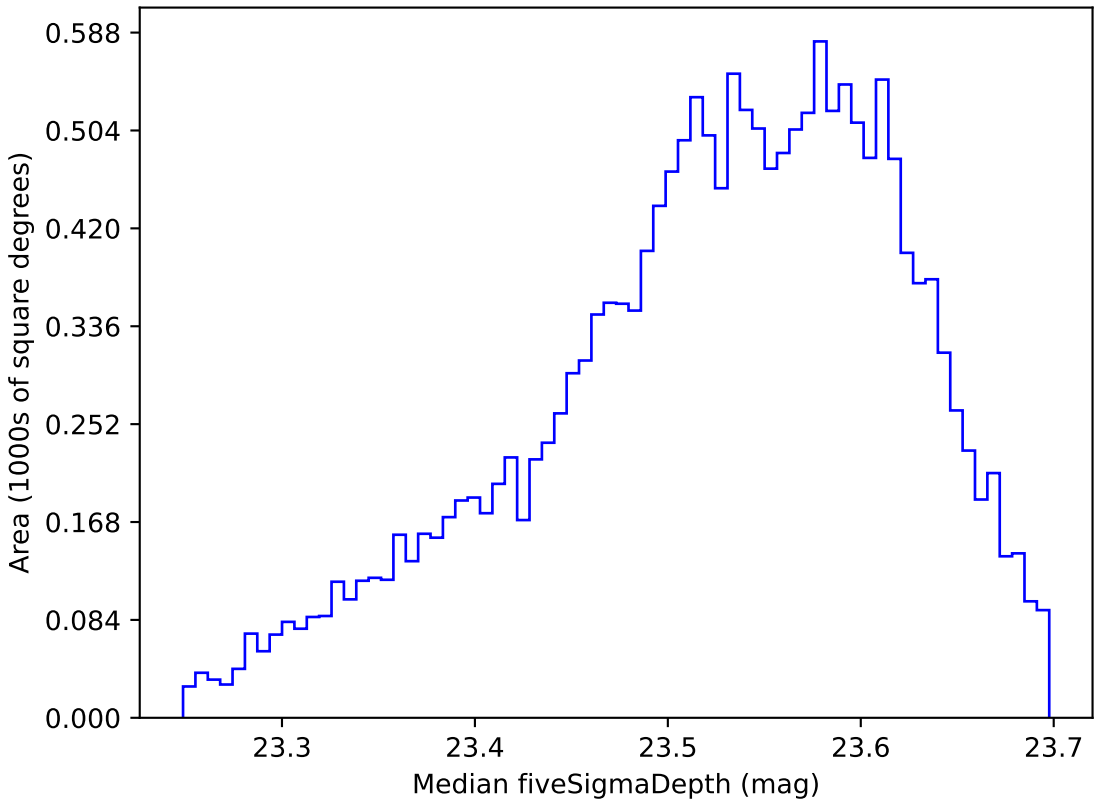
weather_cloudso0v3.5_10yrs WFD i band: Median fiveSigmaDepth
