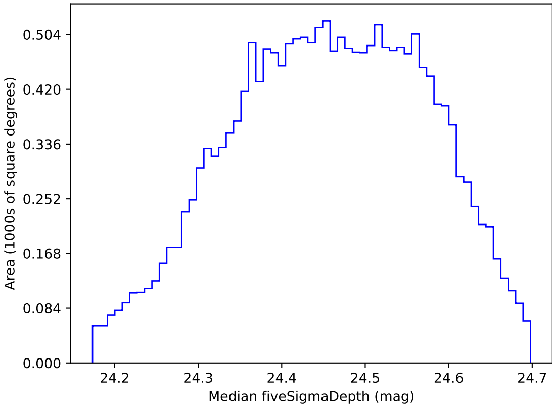
weather_cloudso0v3.5_10yrs WFD g band: Median fiveSigmaDepth
