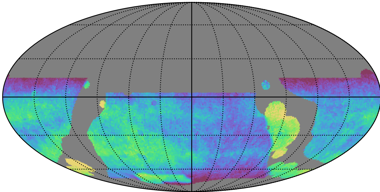
weather_cloudso0v3.5_10yrs WFD all bands: Median fiveSigmaDepth
