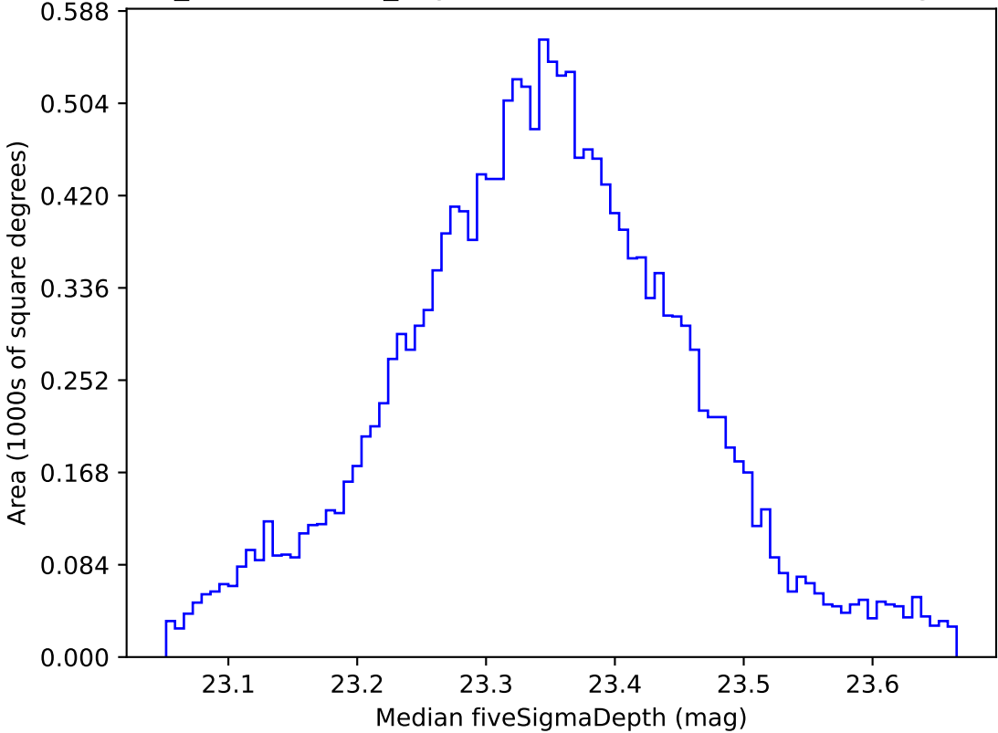
weather_cloudso0v3.5_10yrs WFD all bands: Median fiveSigmaDepth
