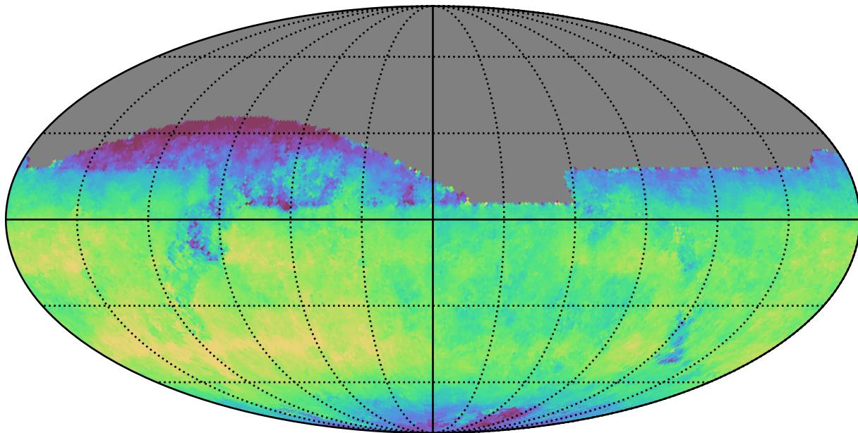
weather_cloudso0v3.5_10yrs All sky z band: Median fiveSigmaDepth
