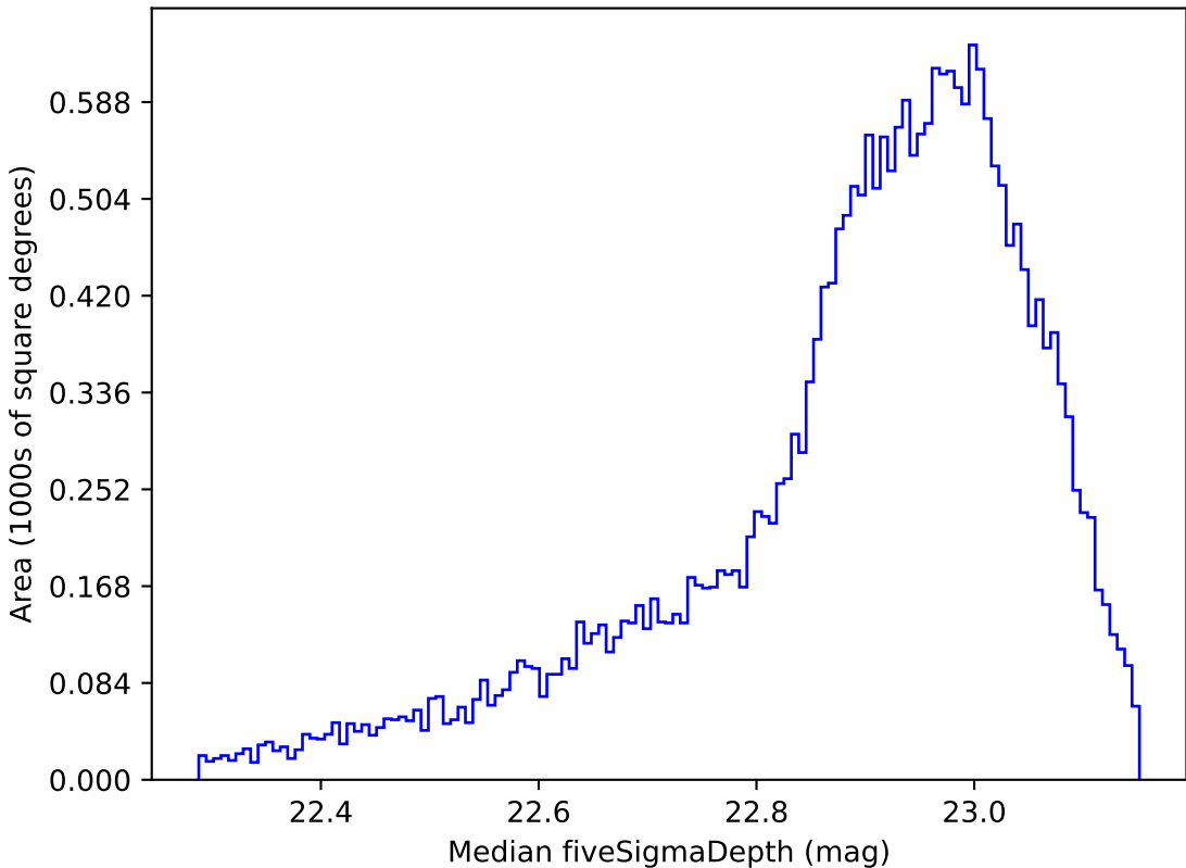
weather_cloudso0v3.5_10yrs All sky z band: Median fiveSigmaDepth
