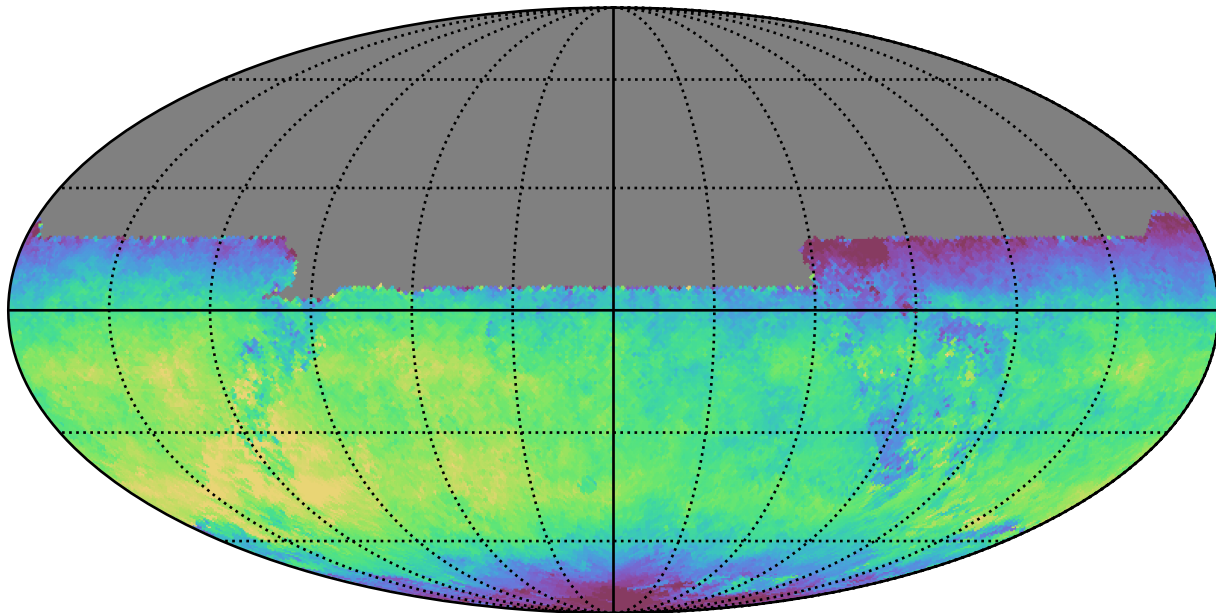
weather_cloudso0v3.5_10yrs All sky y band: Median fiveSigmaDepth
