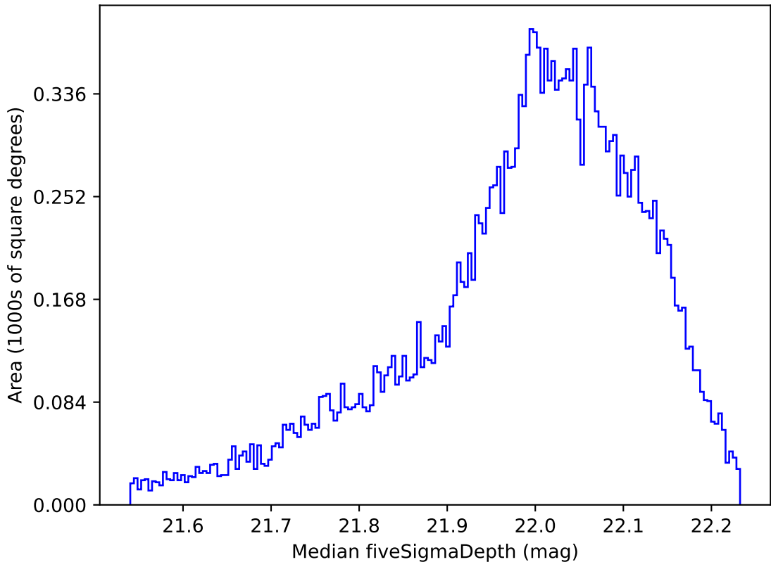
weather_cloudso0v3.5_10yrs All sky y band: Median fiveSigmaDepth
