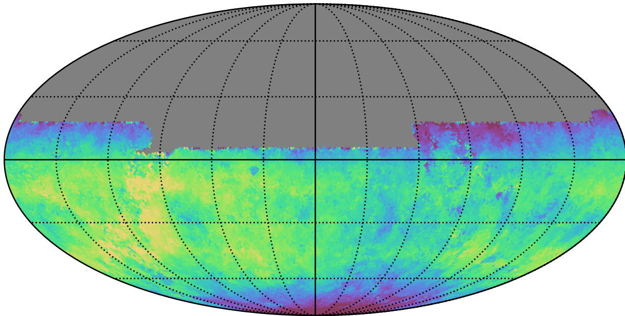
weather_cloudso0v3.5_10yrs All sky u band: Median fiveSigmaDepth
