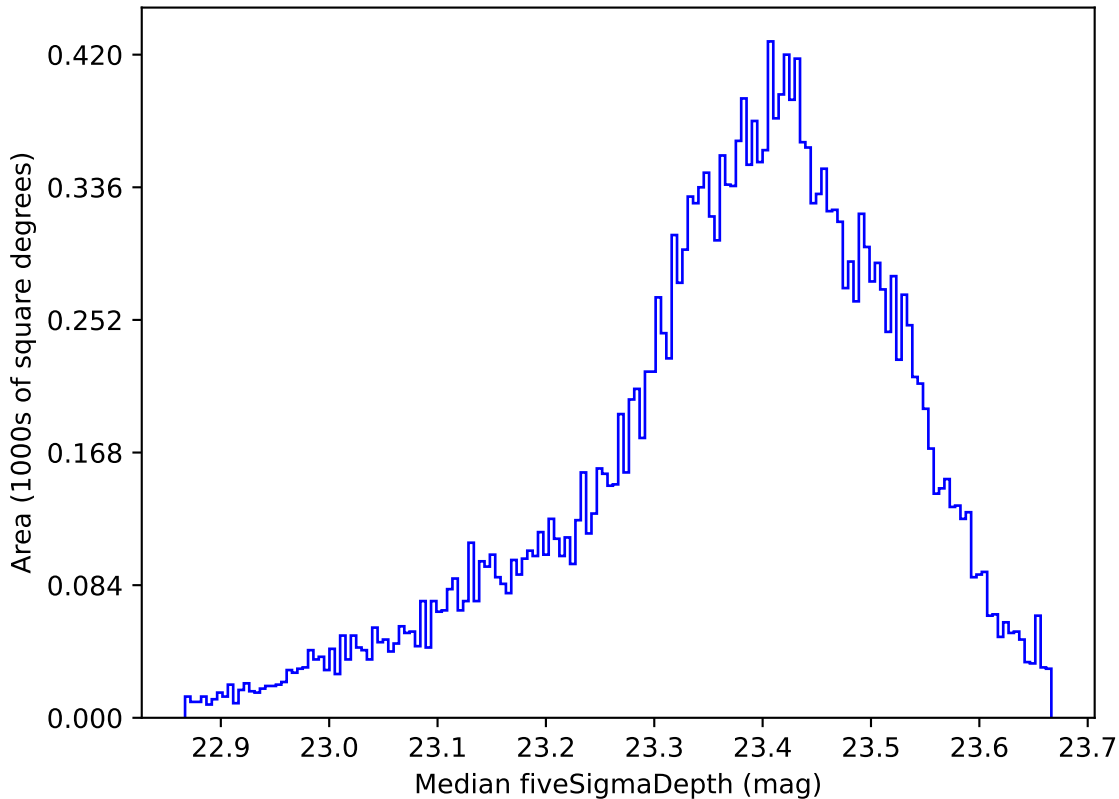
weather_cloudso0v3.5_10yrs All sky u band: Median fiveSigmaDepth
