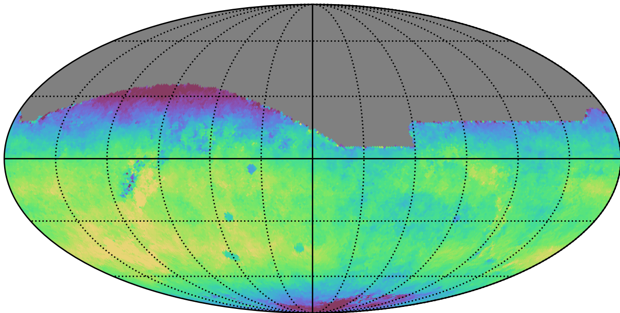
weather_cloudso0v3.5_10yrs All sky r band: Median fiveSigmaDepth
