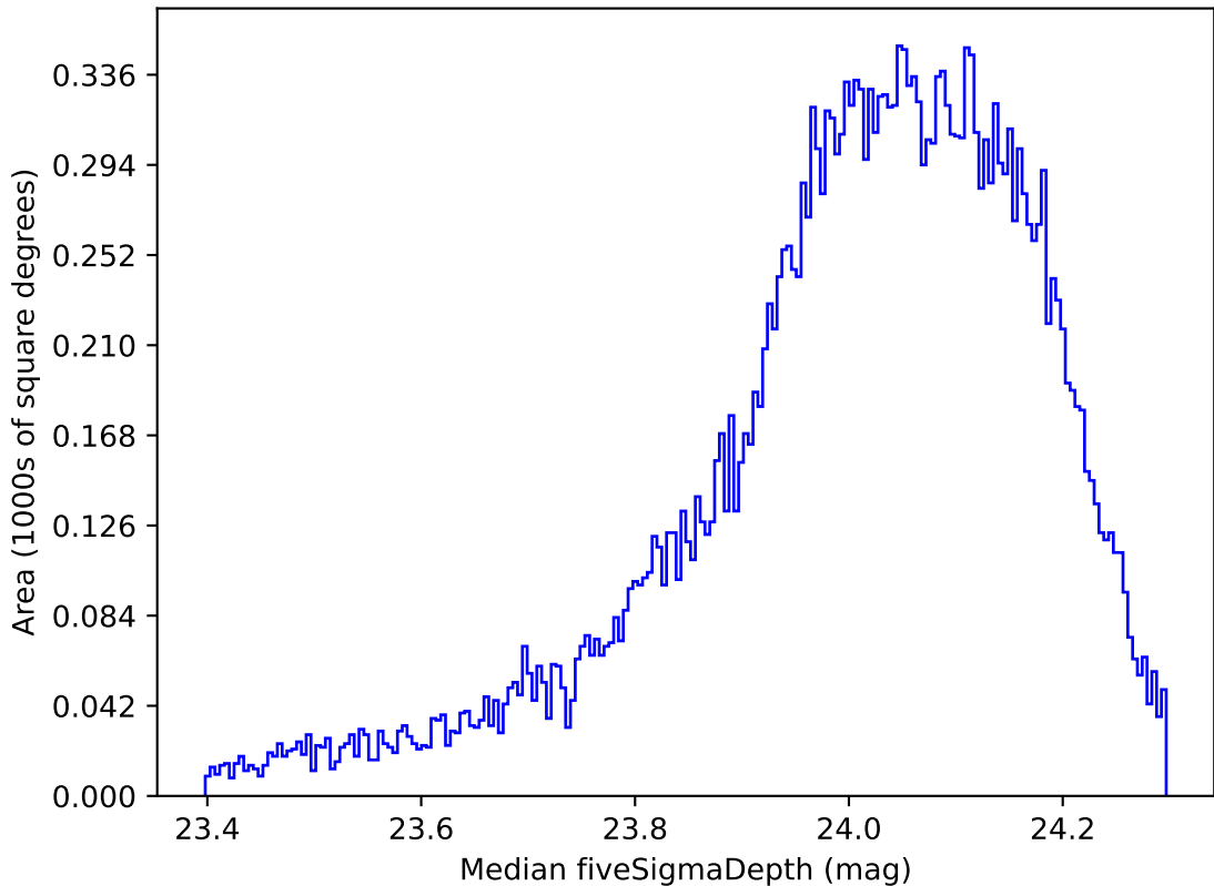
weather_cloudso0v3.5_10yrs All sky r band: Median fiveSigmaDepth
