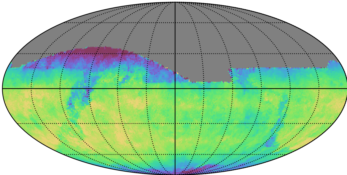
weather_cloudso0v3.5_10yrs All sky i band: Median fiveSigmaDepth
