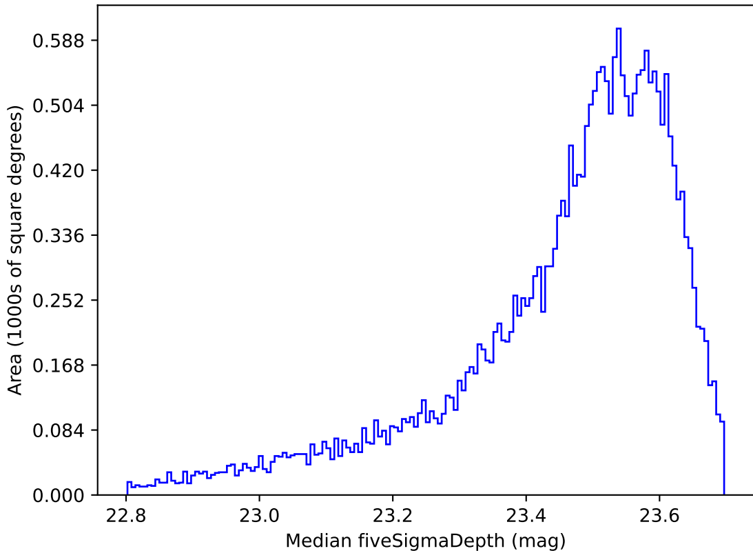
weather_cloudso0v3.5_10yrs All sky i band: Median fiveSigmaDepth
