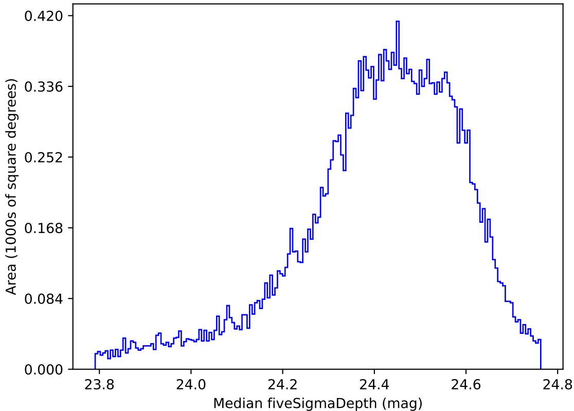
weather_cloudso0v3.5_10yrs All sky g band: Median fiveSigmaDepth
