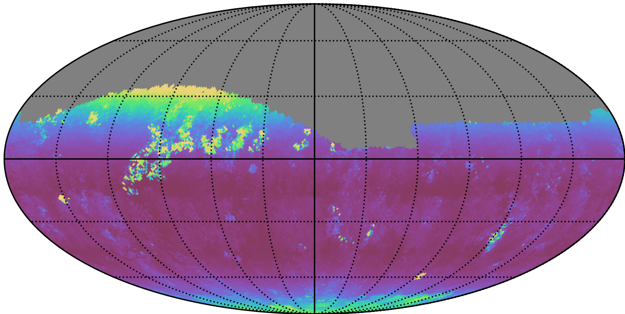
weather_cloudso0v3.5_10yrs Yr 1 z band: Median airmass
