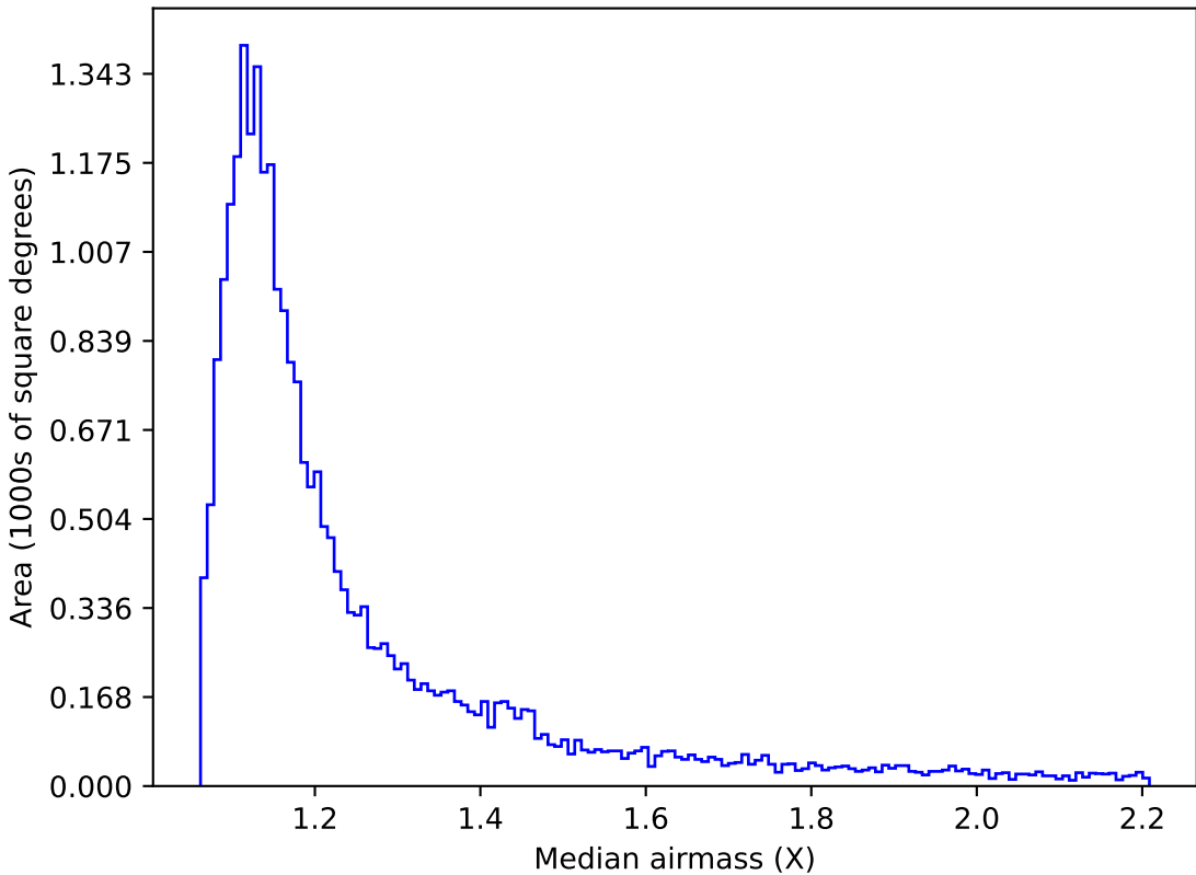
weather_cloudso0v3.5_10yrs Yr 1 z band: Median airmass
