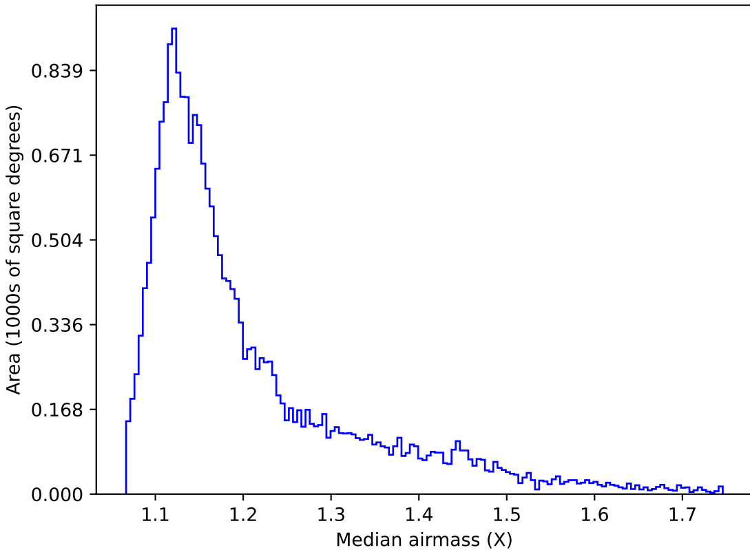
weather_cloudso0v3.5_10yrs Yr 1 y band: Median airmass
