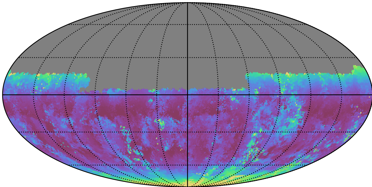
weather_cloudso0v3.5_10yrs Yr 1 u band: Median airmass
