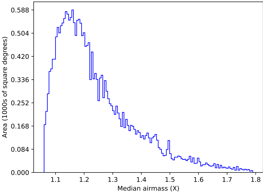
weather_cloudso0v3.5_10yrs Yr 1 u band: Median airmass
