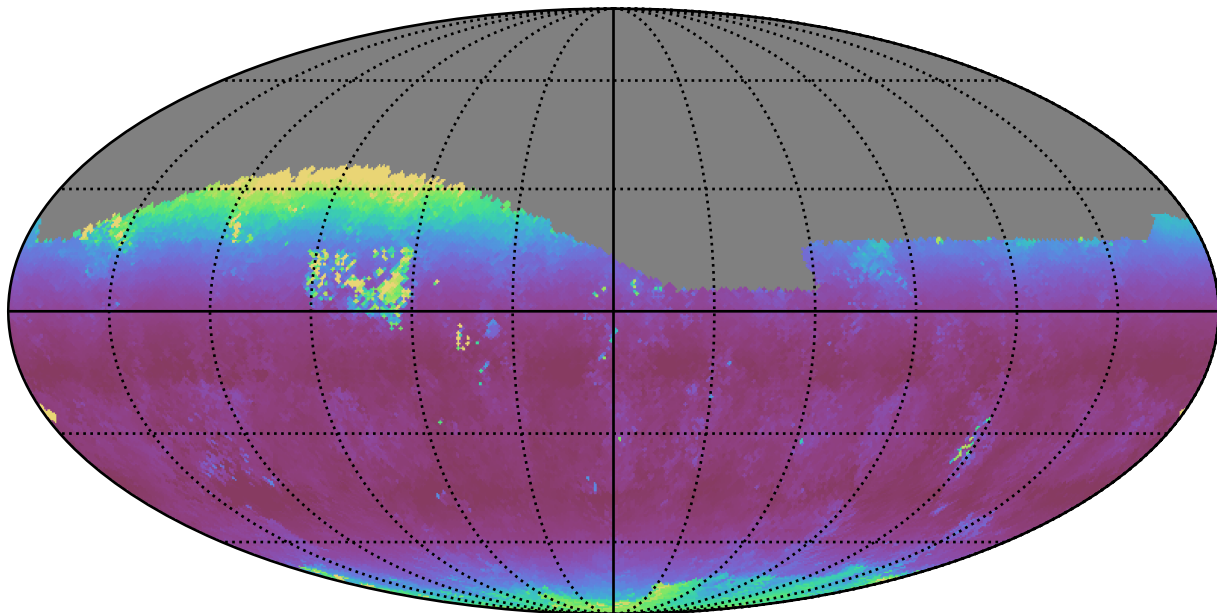
weather_cloudso0v3.5_10yrs Yr 1 r band: Median airmass
